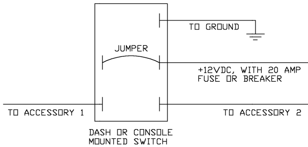
C-SW-3 OFF/ON/ON
