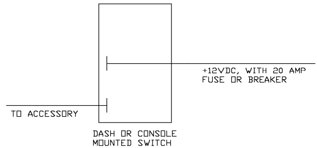
C-SW-4 (ON)/OFF (Momentary)
