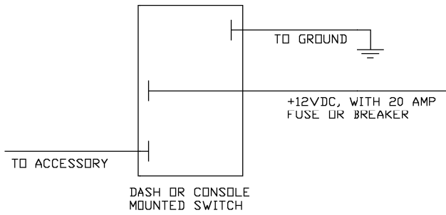
C-SW-1 ON/OFF
