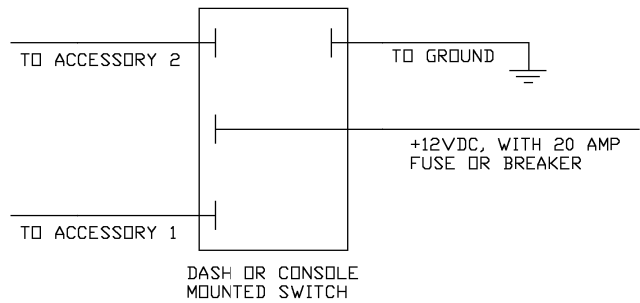
C-SW-2 ON/OFF/ON
