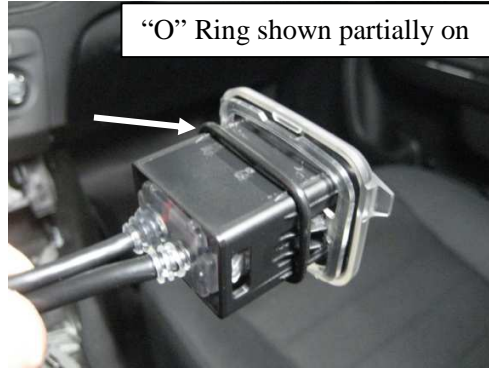
Place # KRM98017 Rubber "O" Ring onto "AUX" socket assembly. Push ring all the way on. This allows for a tight fit when installed.
