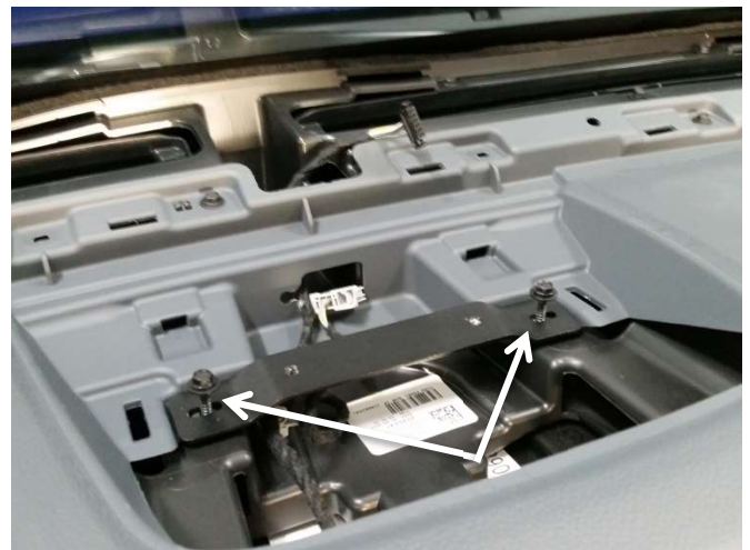
Use OEM hardware and attach upper mounting bracket # CM008207 to OEM inserts.
