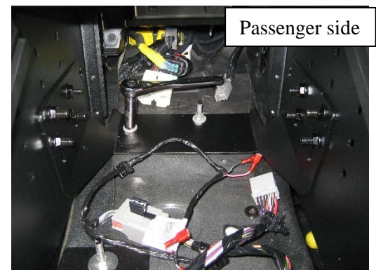
Carefully place console assembly with front floor bracket between seats and onto front O.E.M. floor studs. Loosely attach previously removed OEM nuts or supplied 6mm nuts and washers onto front floor studs.
