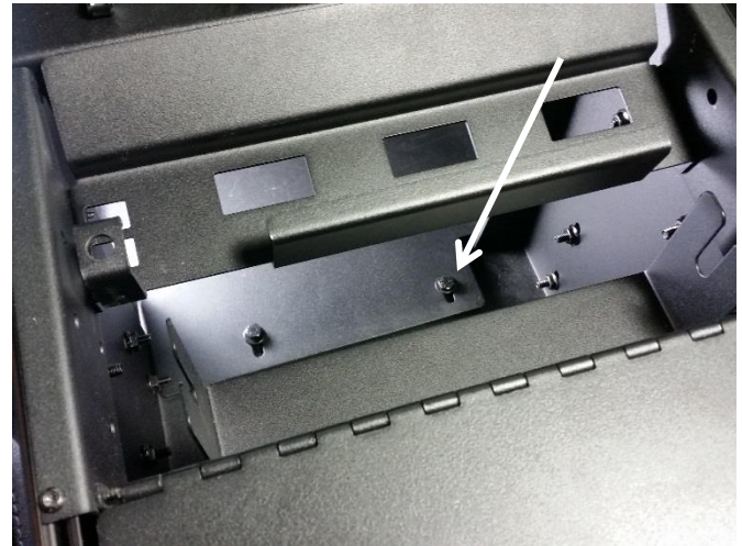
Loosely attach the electrical accessory mounting plate to the console "U" bracket with 1/4" x 3/4" Hex bolts and washers.
