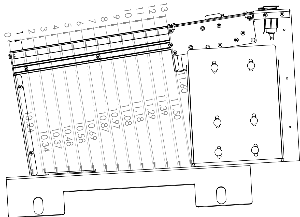
PS 3.3" WIDE SECTION
