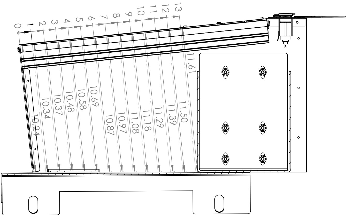
PS 3.3" WIDE SECTION
