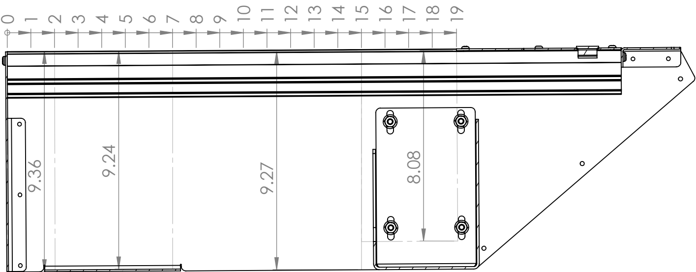
PS 3.3" WIDE SECTION
