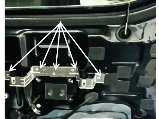
Remove factory metal bracket by drilling out five (5) rivets. NOTE: Make sure the window is up before drilling into the door panel.
