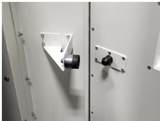
Attach door stop "Socket" and bracket assembly to door frame using #8 x 3/4" Phillips machine screws and nuts. Bracket mount holes may need to be drilled in rear bulkhead.
