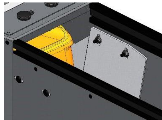
Loosely attach housing to brackets with 1/4" x 3/4" carriage bolts and serrated nuts. Double check positioning.
