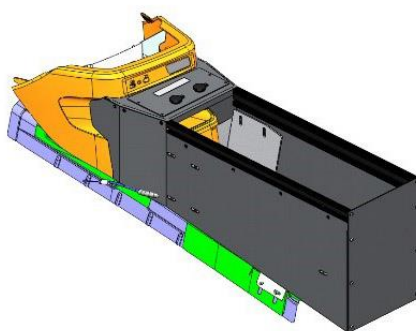
Slide main console housing onto floor brackets. Connect wiring to Accessory Power outlets (APO's / 12 volt sockets)
