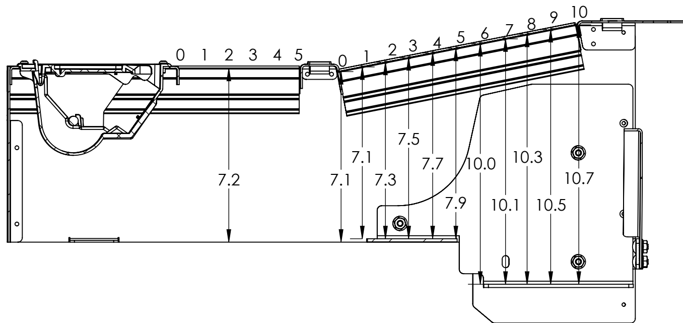
9" WIDE SECTION
